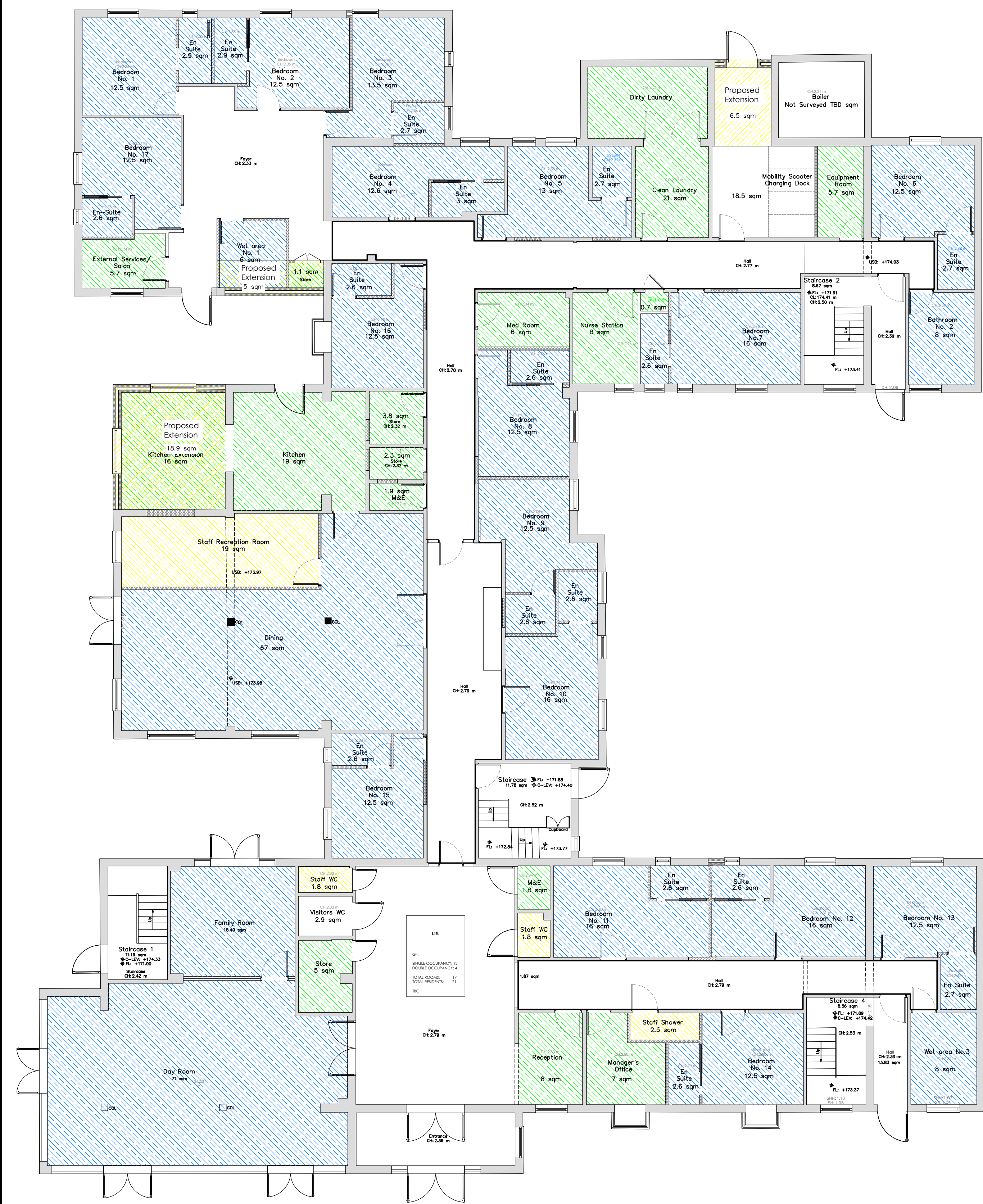
Ground Floor Plan as PROPOSED 1:100
