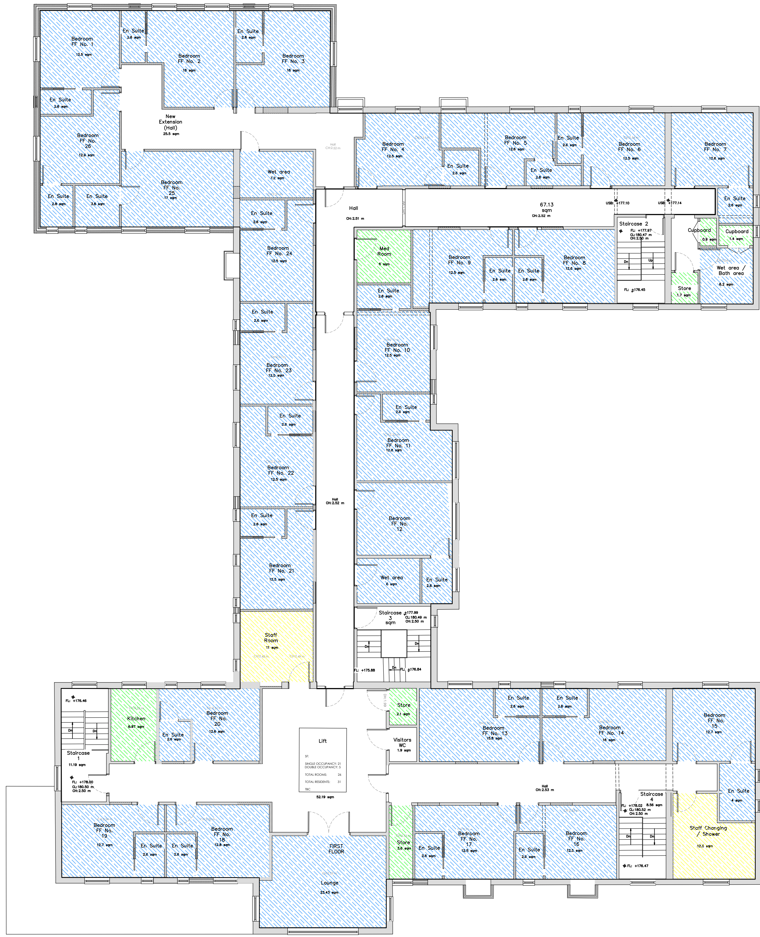
Second Floor Plan as PROPOSED 1:100
