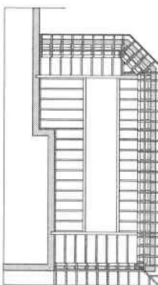
Combined Flat And Pitched Roof Plan
