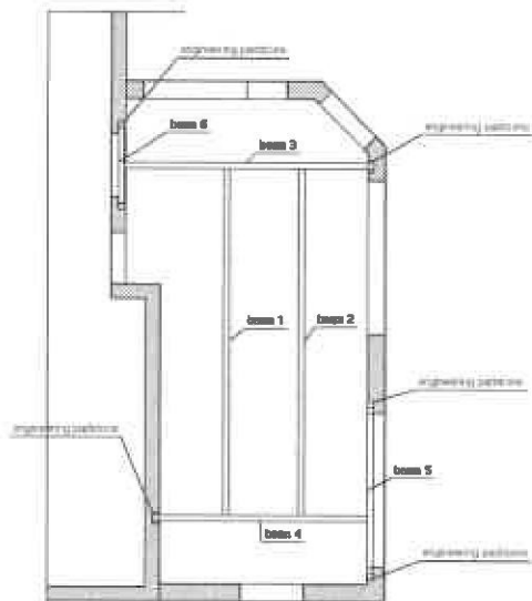
Steelwork Plan
