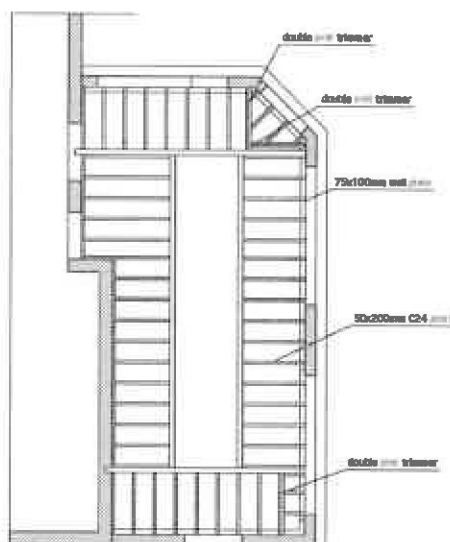
Flat Roof Plan
