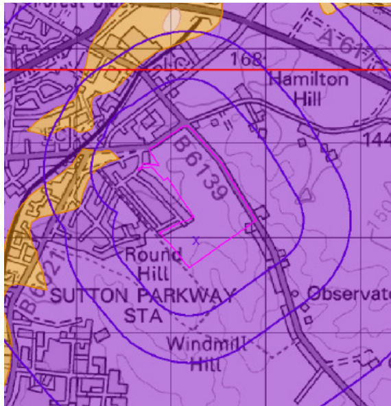
Extract showing the solid geology Principal aquifer below the site and below the surrounding area within 500 m of the site.
